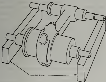
FIGURE 10-22. Checking connecting rod squareness.
